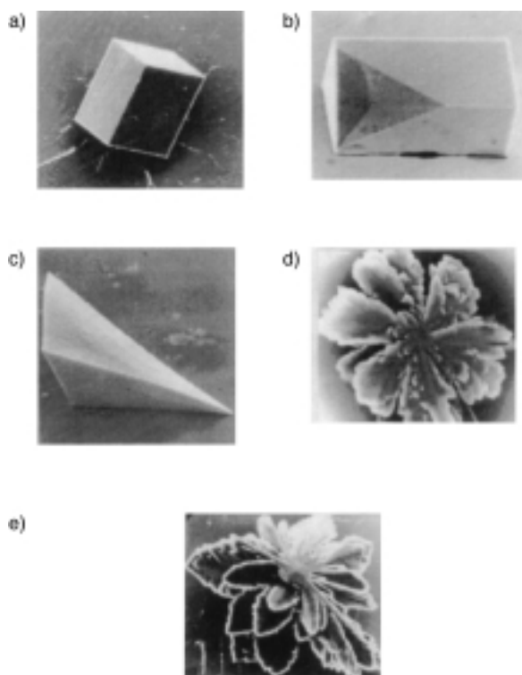
Figure 2. a) Calcite control crystal, 1 cm = 5 μm; b) {01.2}-oriented calcite grown under monolayer 1 · 2 (R = CH 2 CH 2 CO 2 H), 1 cm = 5 μm; c) [001]-oriented calcite grown under monolayer 1 · 2 (R = CH 2 CH 2 CH 2 OPO 3 H 2 ), 1 cm = 15 μm; d) [001]-oriented vaterite and e) < 11.0 > oriented vaterite, both grown under monolayer 1 · 2 (R = CH 2 CH 2 CH 2 NH 3 + Cl - ), 1 cm = 25 μm.
